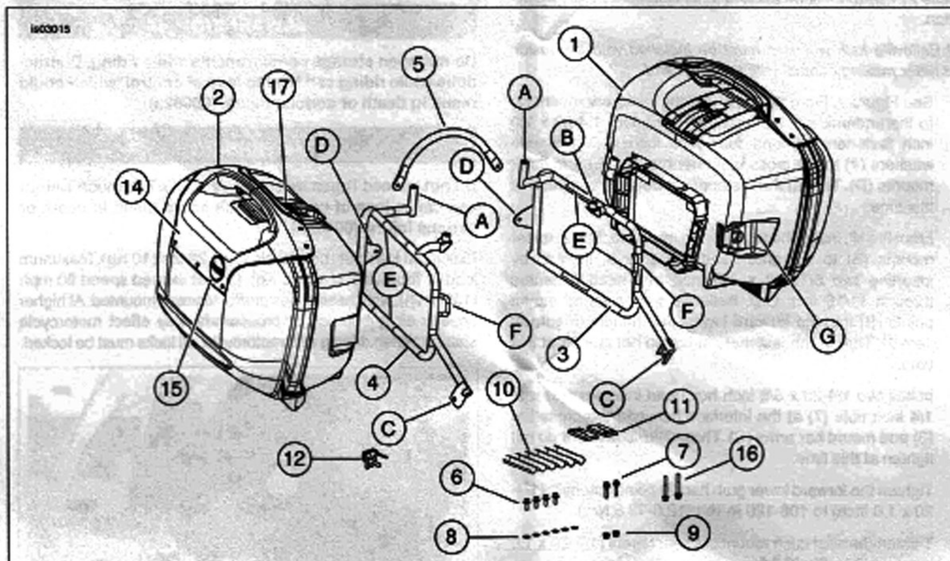
Figure 6. Service Parts: Ulysses Sidecase
