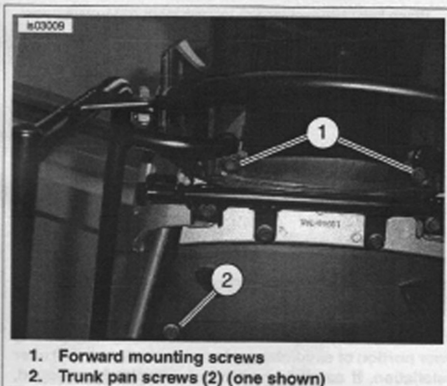
Figure 1. License Plate and Trunk Pan Screw Removal
