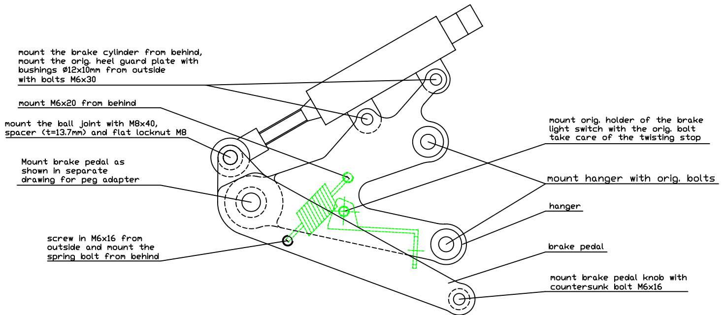
rear set CBR 900 RR '00-01 mounting drawing, brake
