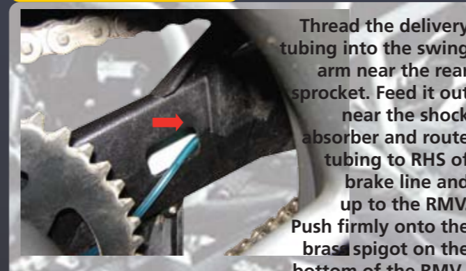
Triumph Tiger 800XC mount on right hand side
