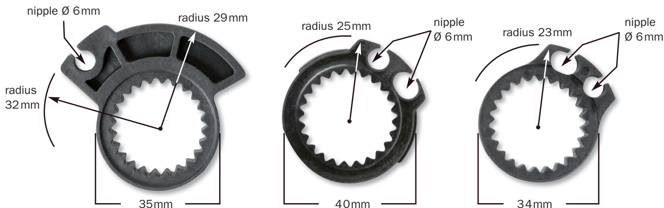
All mounts for 1.5 mm Bowden cables!
